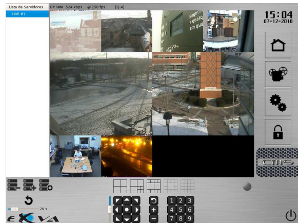
Fig. 4: Software CMS
