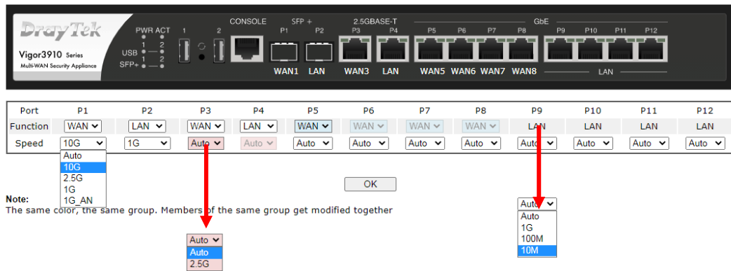
Port Setup
