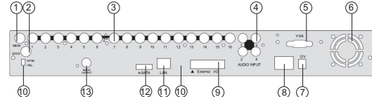
Back Panel Layout
